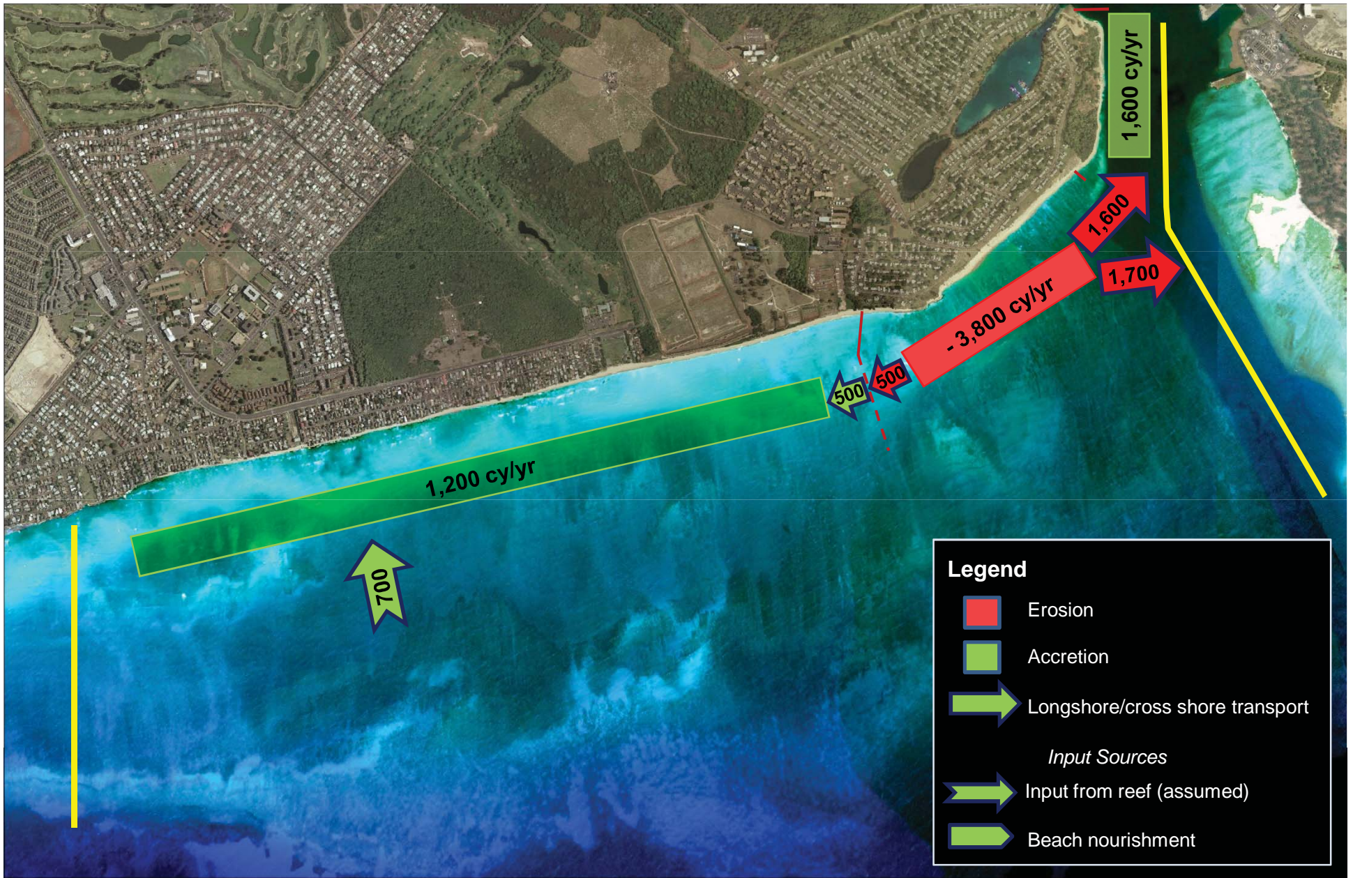
Figure 24 Preliminary Sediment Budget for Iroquois Point Analysis dated December 2009
