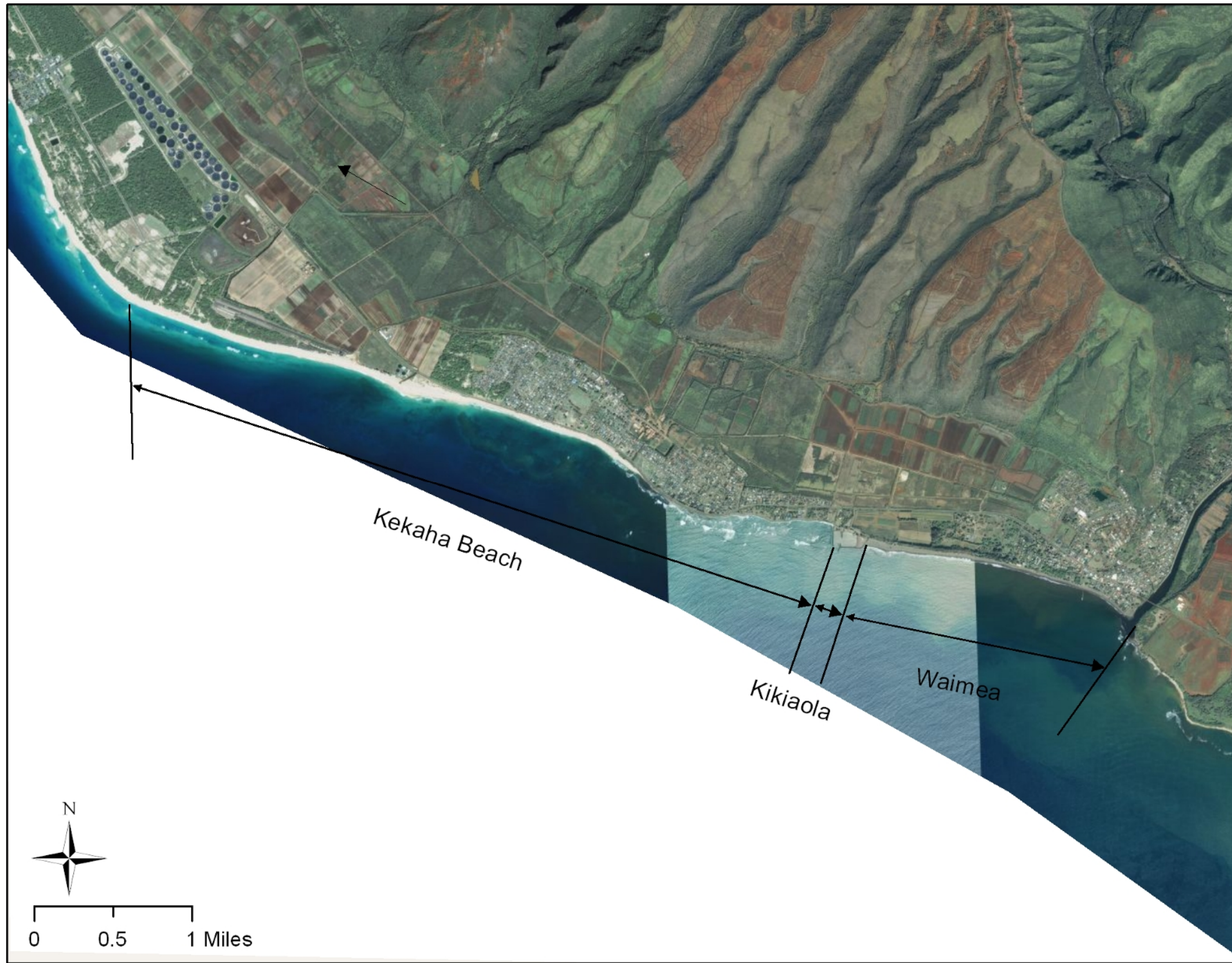
Figure 28. Kekaha Region Littoral Cells
