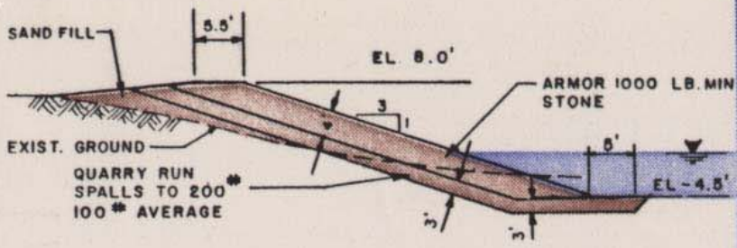
REVETMENT TYPICAL SECTION
