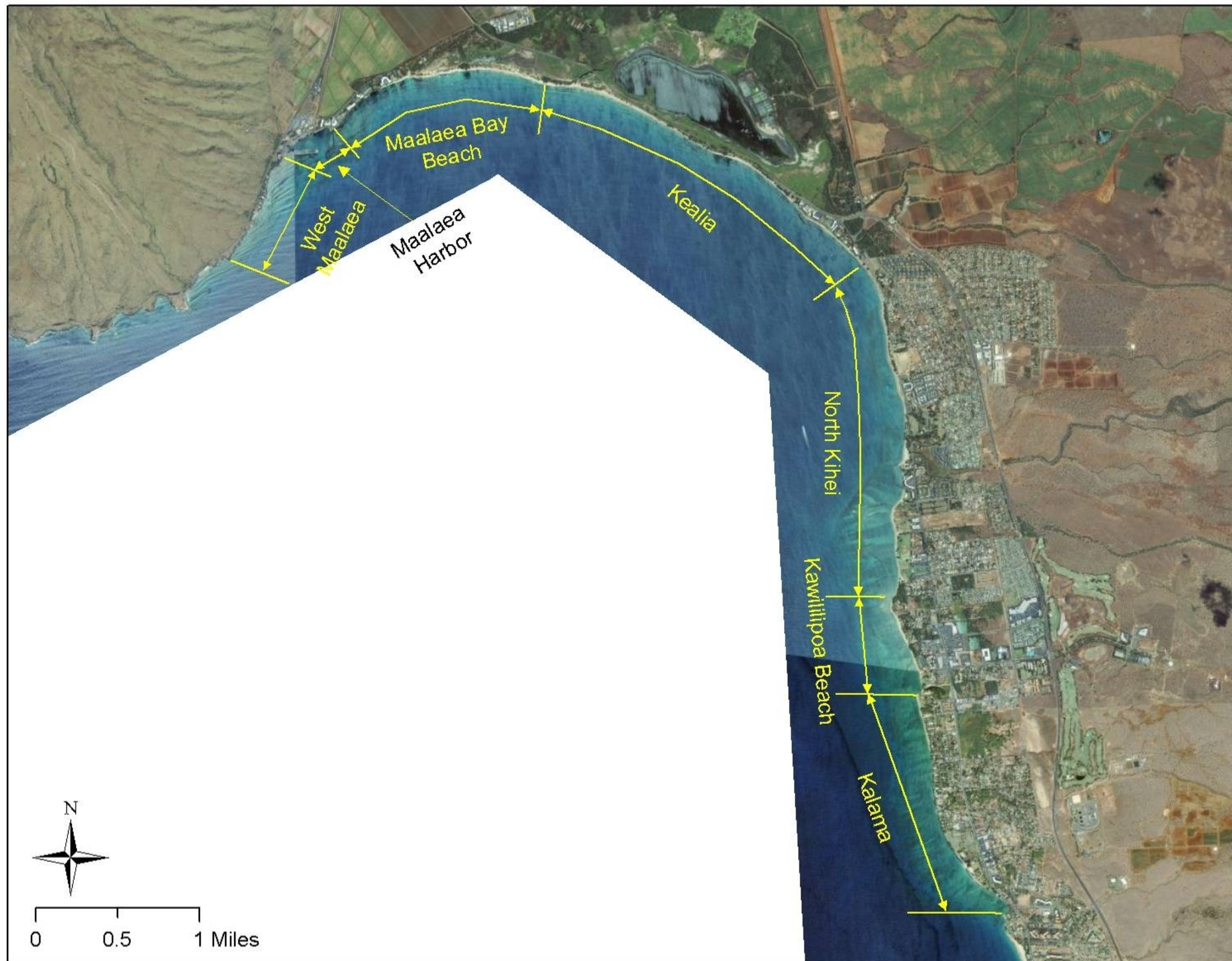
Figure 32. Kihei Region Littoral Cells
