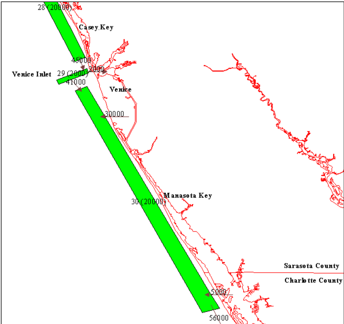
Figure 6. Southern Sarasota County Sediment Budget
